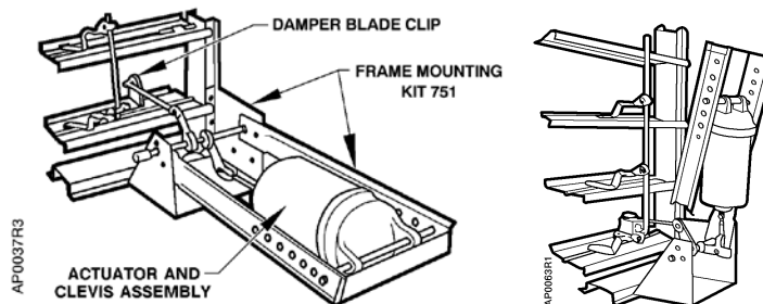
Figure 5. One-section Damper.
