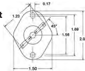
Limit Control Switches – Manual Reset (Flanged Surface Mount – 36T)
