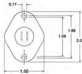
Limit Control Switches – Auto Reset (Large Flanged Airstream – 44T Low Voltage)
