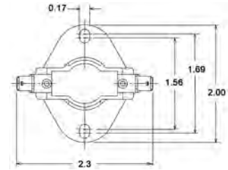
Limit Control Switches – Auto Reset (Large Flanged Airstream – 64T Two Pole)
