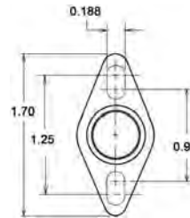
Limit Control Switches – Manual Reset (Special Small Flanged Airstream – 36T)
