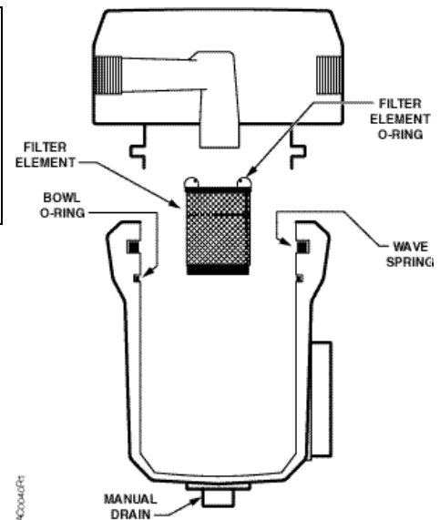
Figure 2. Filter Element Replacement.
