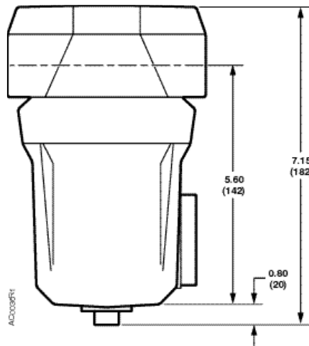
Figure 1. Air Line Filter Assembly Dimensions in Inches (Millimeters).
