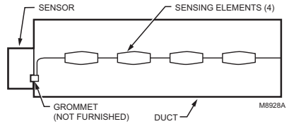
Fig. 3. Duct cross section showing method of installing C7021J, C7023J/C7031J/C7041J in a multizone system.
