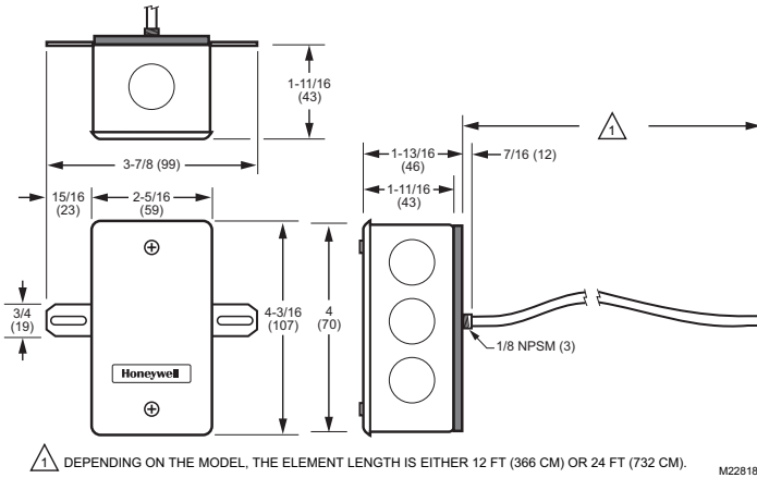
Fig. 4. C7021R, C7023R, C7041R dimensions in in. (mm).
