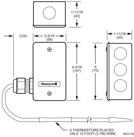
Fig. 1. C7021J, C7023J, C7031J, C7041J dimensions in in. (mm).
