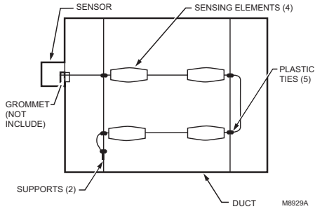
Fig. 2. Duct cross section showing method of installing C7021J, C7023J, C7031J, C7041J Averaging Electronic Sensor.
