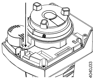
Figure 20. Step 2—Check LED.
