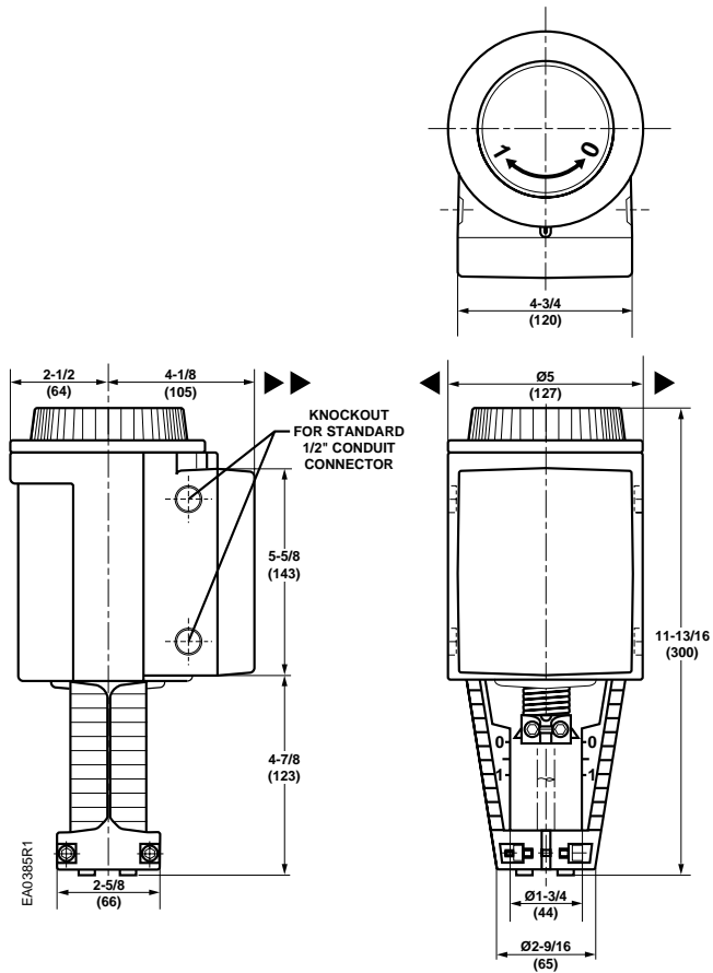
Figure 19. Dimensions of SKD Actuator.
