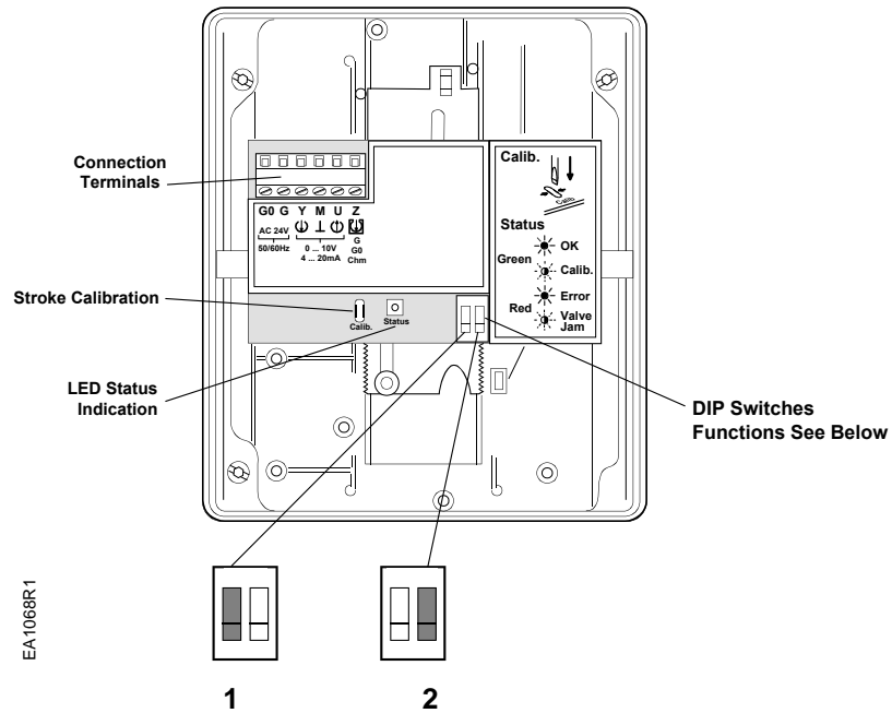
Figure 12. SKD Electronic Features.
