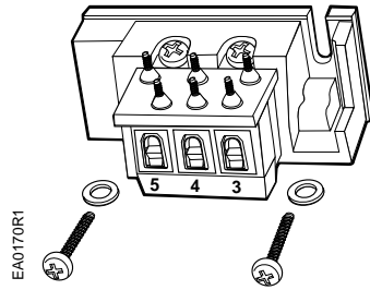
Figure 1. Auxiliary Switch.
