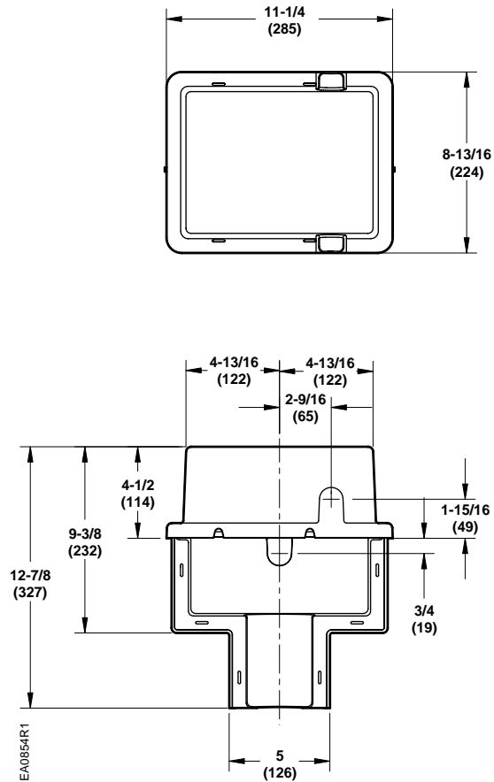
Figure 18. Dimensions of 599-10071 Weather Shield in Inches (Millimeters).
