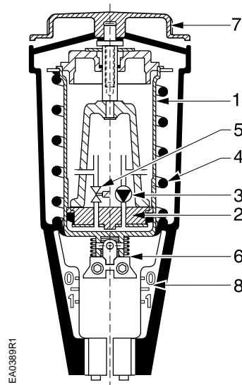
Figure 5. SKD Details.
