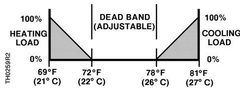
Figure 4. TH 193 HC Operating Characteristics.
