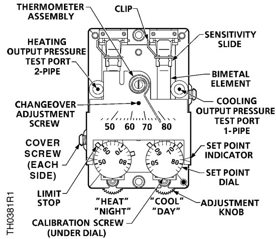
Figure 6. TH 193 HC Thermostat Details.
