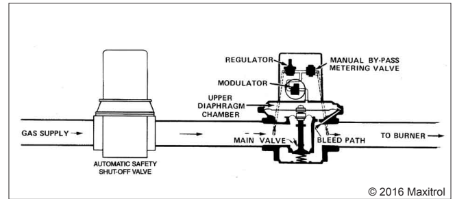
Figure 7 : MR Valve-Modulator/Regulator Valve
