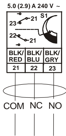
Figure 20: Optional Auxiliary Switch Wiring
