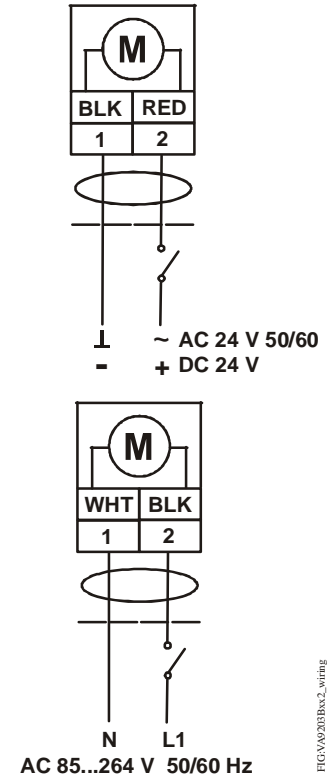
Figure 19: Control Wiring Diagrams
