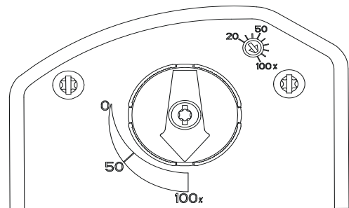
Figure 22: Switch Trip Point Settings
