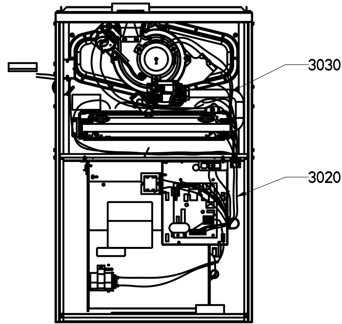
WIRE ROUTING
