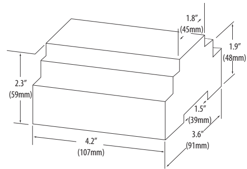
Mounting Diagram
