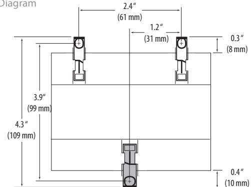
Mounting Diagram
