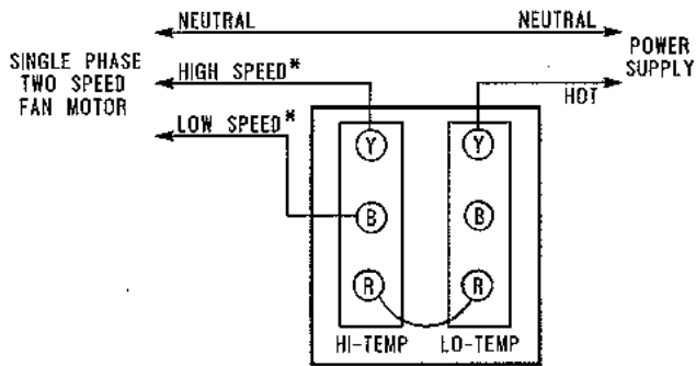
Fig. 5 — Typical wiring hookup for two-speed fan motors provides high speed, low speed and "Off" control.
