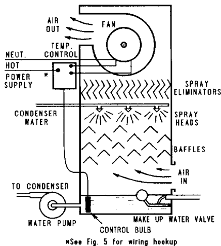
Fig 4: Wiring hookup and installation of the A28MA-1 Cooling Tower Fan Control with a forced draft cooling tower.
