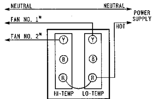
Fig. 6 — Typical wiring hookup for two fan control provides dual fan, single fan and "Off" control.
