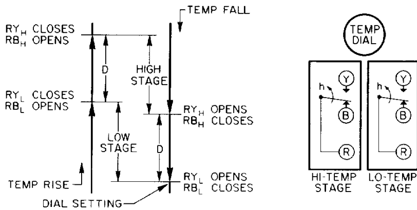
Fig. 3: Switching action of the two-stage control is illustrated above. RB H , RY H indicates HI-TEMP stage; RBL, RYL indicates LO-TEMP stage. "D" represents the differential between stages.
