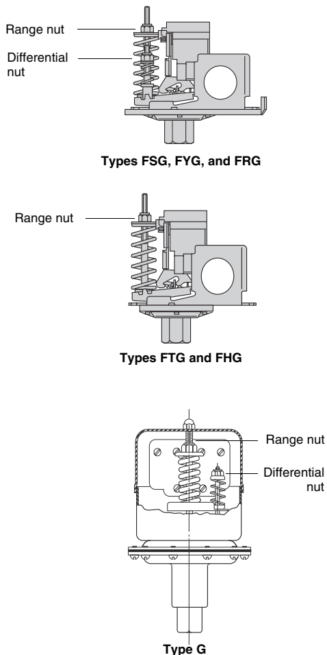
Figure 1: 9013F/9013G Pressure Switches With Adjustable Differential
